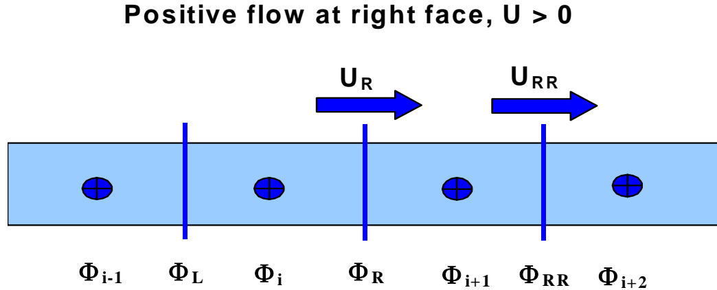
Figure A-26. Definition sketch for variable velocity.
