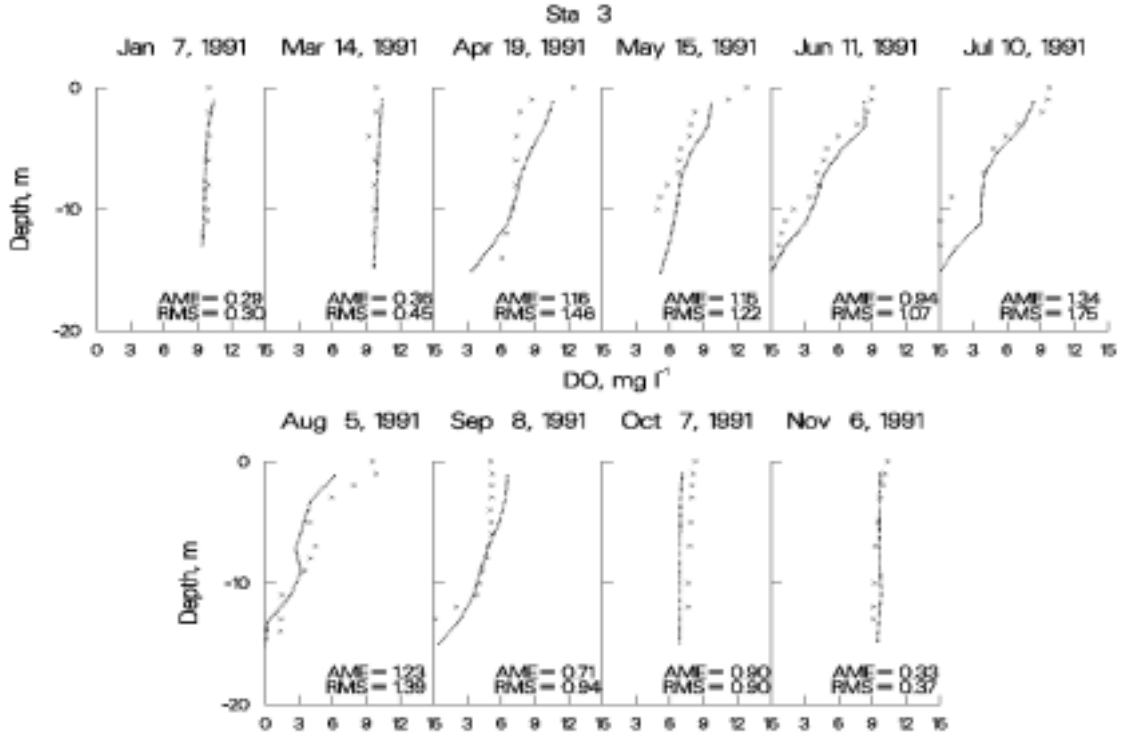
Figure 28. Weiss Reservoir computed vs. observed DO.
