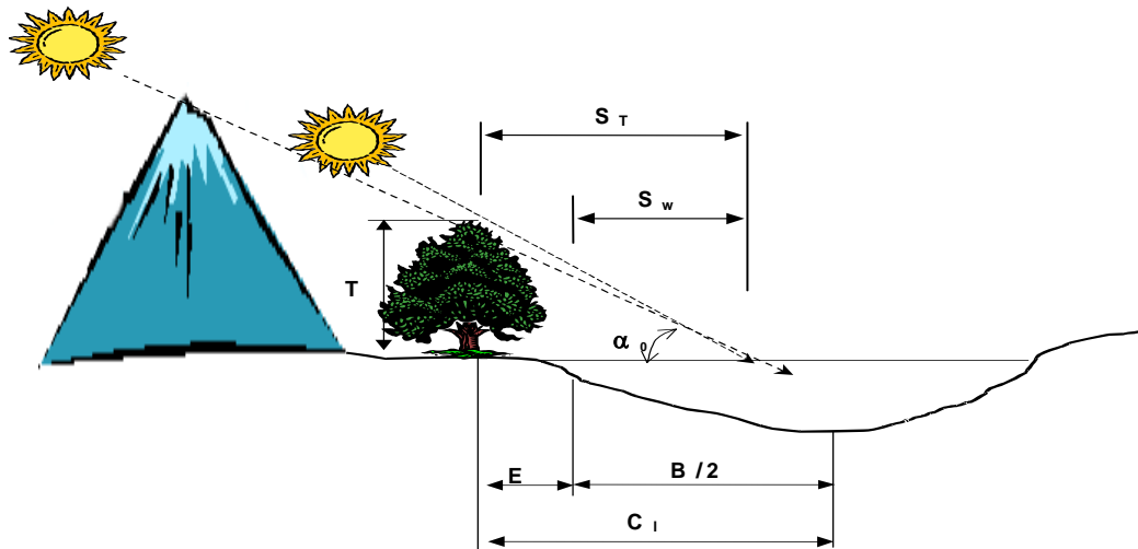
Figure A-51. Schematic of topographic and vegetative shading, solar altitude ( \alpha_0 ), and vegetation height ( T ) and their affect on shadow length.
